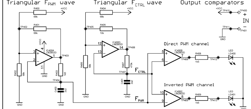
4. Two channel alternating PWM generator
