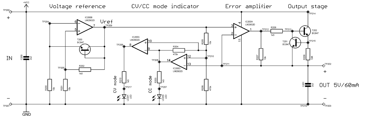
2. Fixed voltage regulator with overcurrent limiter and CV/CC mode indicator
