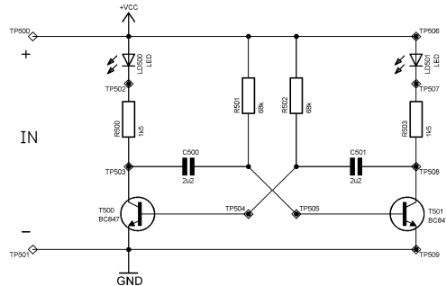
5. Astable flip-flop
